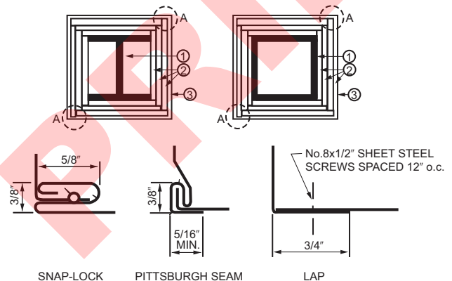
FIGURE 722.5.1(2) GYPSUM-PROTECTED STRUCTURAL STEEL COLUMNS WITH SHEET STEEL COLUMN COVERS
