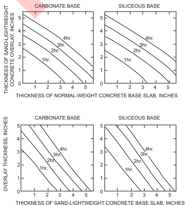
FIGURE 722.2.2.2 FIRE-RESISTANCE RATINGS FOR TWO-COURSE CONCRETE FLOORS
