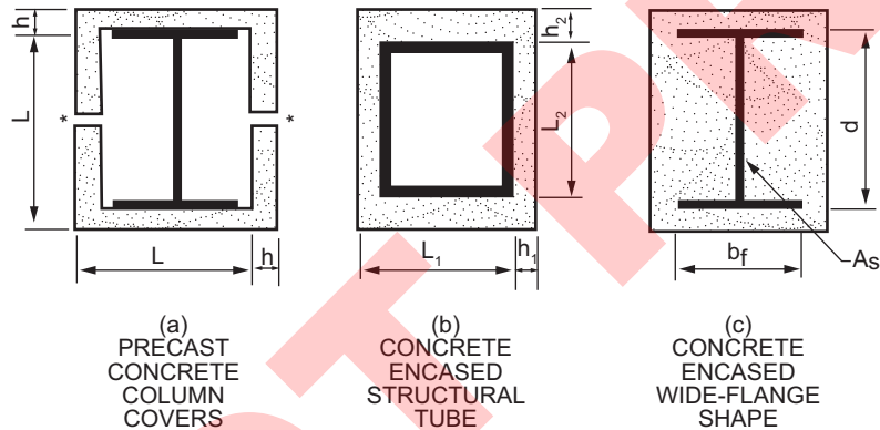
FIGURE 722.5.1(6) CONCRETE PROTECTED STRUCTURAL STEEL COLUMNS a, b
