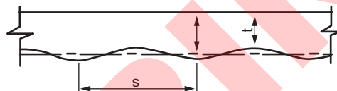
FIGURE 722.2.2.1.3 SLABS WITH RIBBED OR UNDULATING SOFFITS
